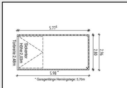
TYP XS Betonfertiggarage
